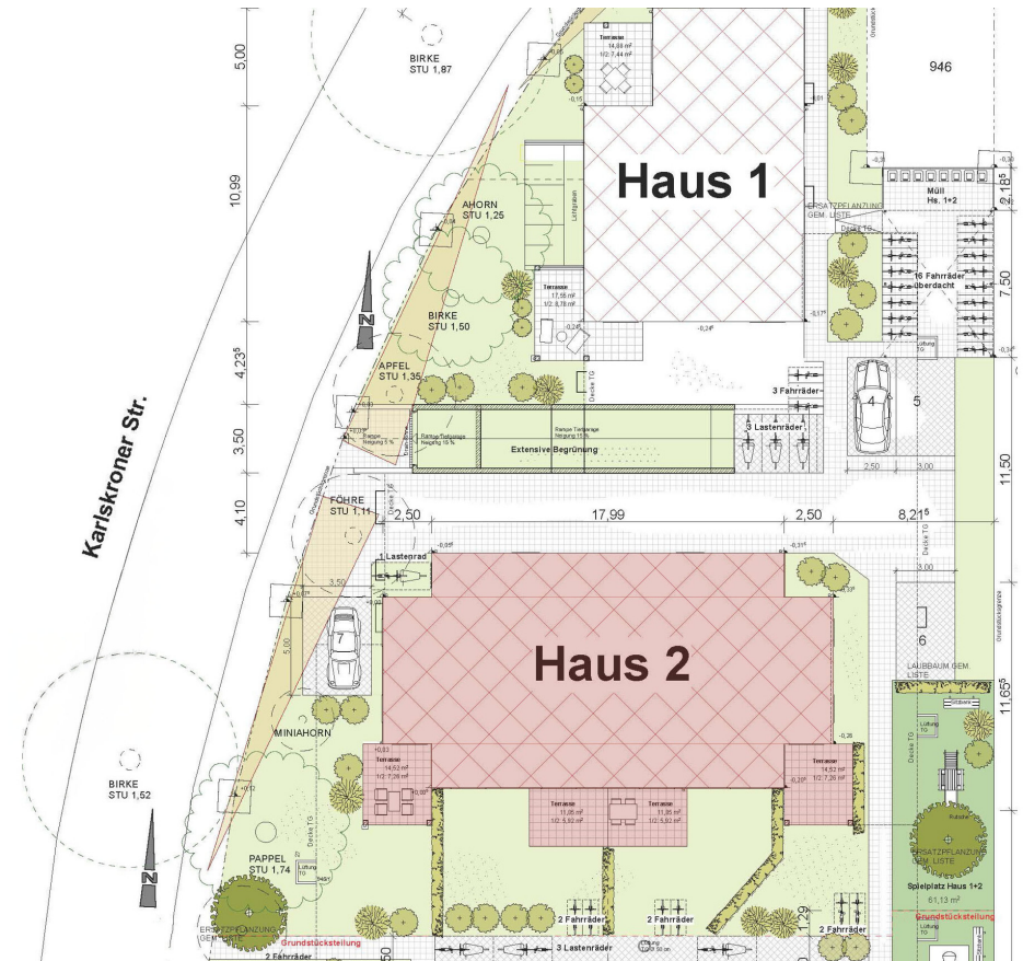
BI-25-05-W14-Lageplan_H1-2
