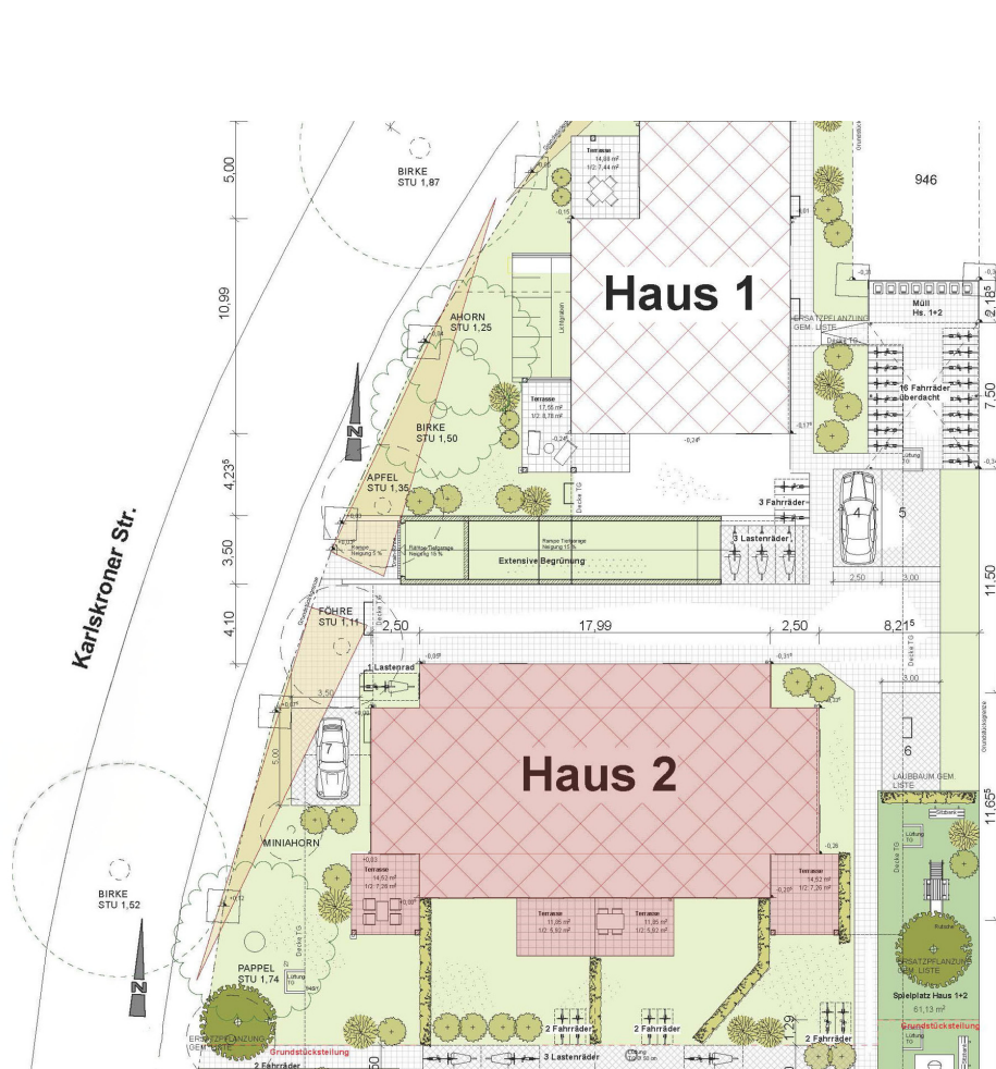
BI-25-05-W14-Lageplan_H1-2
